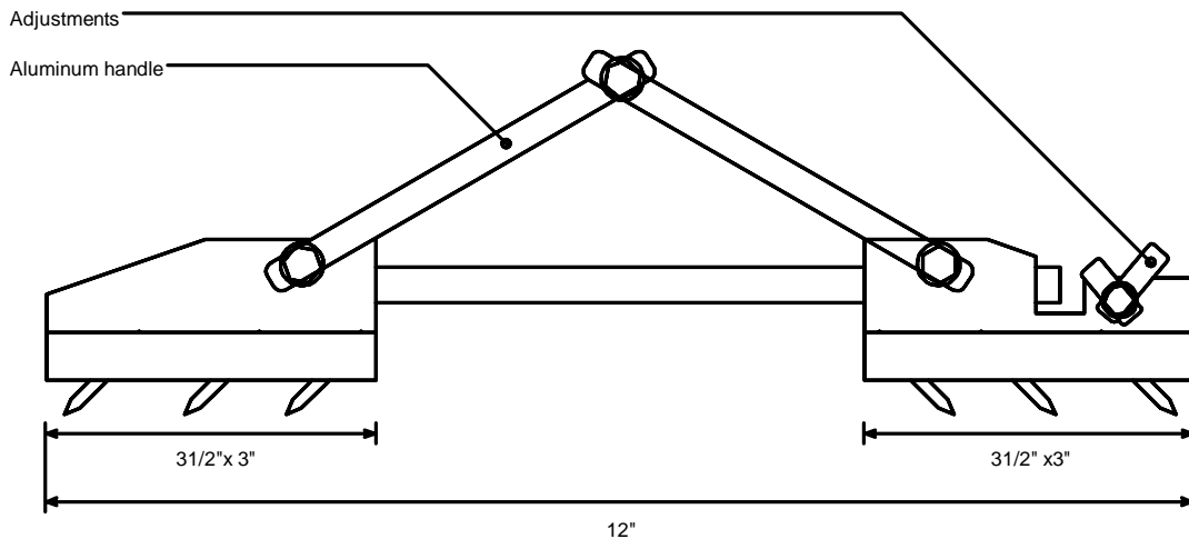
CLAW TYPE LIFTER FOR CUT PILE CARPETS
