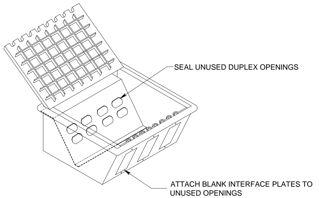
POWER, VOICE, AND DATA DISTRIBUTION BOX
